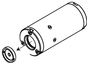
Outline picture and drawing of PCB4S BBO Pockels cell
