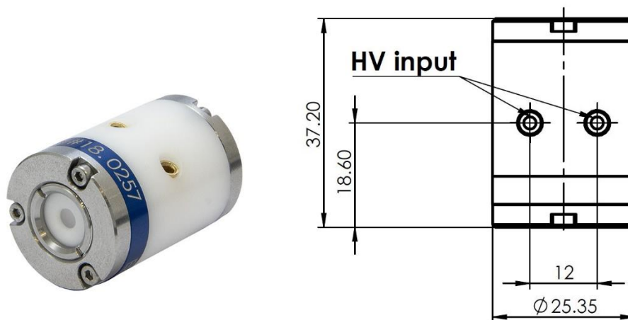
Outline picture and drawing of PCB4S BBO Pockels cell
