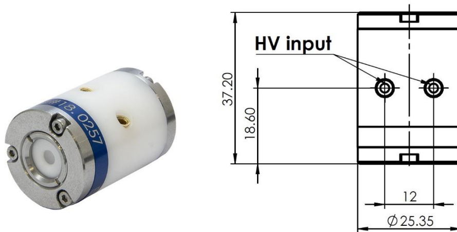
Outline picture and drawing of PCB3S BBO Pockels cell
