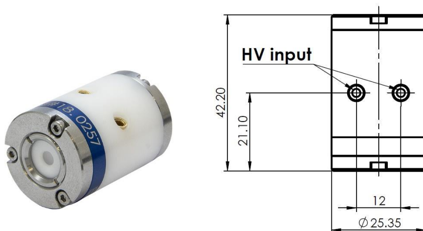
Outline picture and drawing of PCB3S/25 BBO Pockels cell
