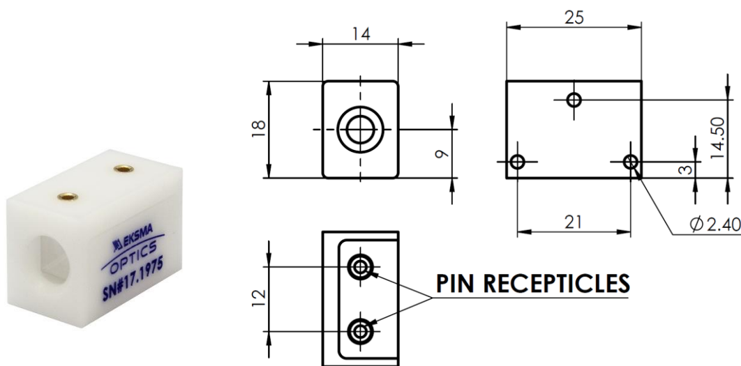
Outline picture and drawing of PC5S DKDP (KD*P) Pockels cell
