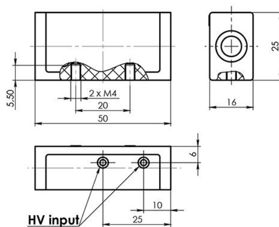
Outline picture and drawing of PC5D DKDP (KD*P) Pockels cell
