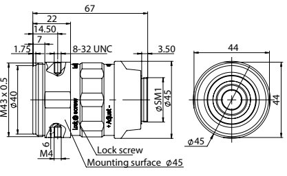
Model for 1.5X and 2X expanders
