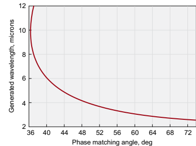
Type 2 DFG ( e-o=e ) in AGS. DFG of signal and idler generated in BBO pumped at 800 nm
