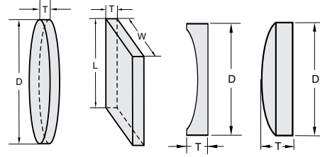
Drawings of flat round, flat rectangular and spherical mirrors
