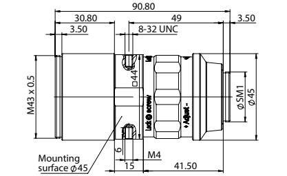
Model for 3X and 5X expanders
