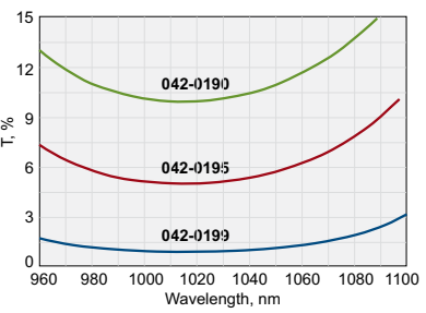
042-0199. PR = 99±0.5% @ 1030 nm, T = 1±0.5% 042-0195. PR = 95±2% @ 1030 nm, T = 5±2% 042-0190. PR = 90±2% @ 1030 nm, T = 10±2%
