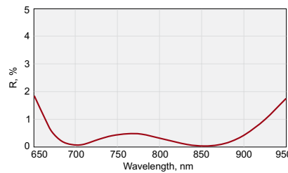
Reflectivity @ 700-900 nm
