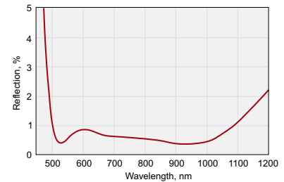
R&lt;1.5% @ 500-1100 nm, AOI=0°
