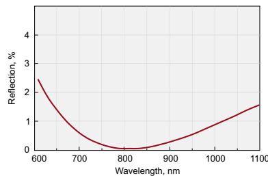
R&lt;0.8% @ 700-900 nm, AOI= 0°
