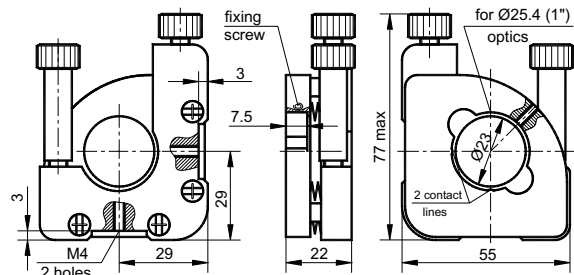
Positioning mount 840-0193
