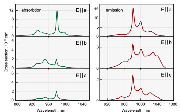
Absorption and emission spectra of Yb(5%):KGW
