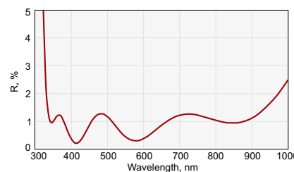
Reflectivity @ 350-900 nm
