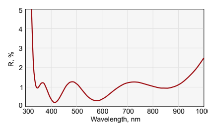
Reflectivity @ 350-900 nm
