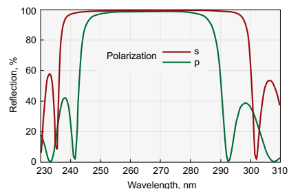
HR>99% @ 257-275 nm, AOI=45°
