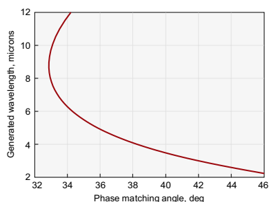
Type 1 DFG (e-o-o) in AGS. DFG of signal and idler generated in BBO pumped at 800 nm
