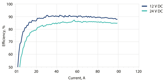
uniLDD efficiency. 12 V and 24 V DC power, 2 V junction + 10 MΩ series R load
