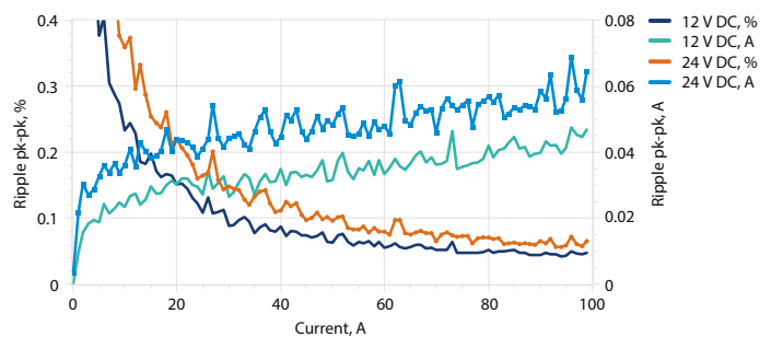
uniLDD ripple current. 12 V and 24 V DC power, 2 V junction + 10 MΩ series R load
