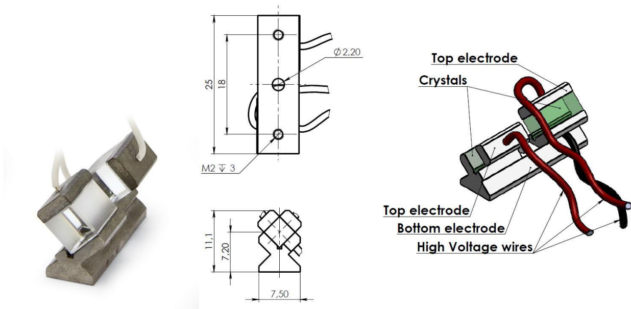
Outline picture and drawing of PCK4-O KTP Pockels cell
