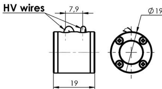
Outline picture and drawing of D-mini/8 DKDP (KD*P) Pockels cell
