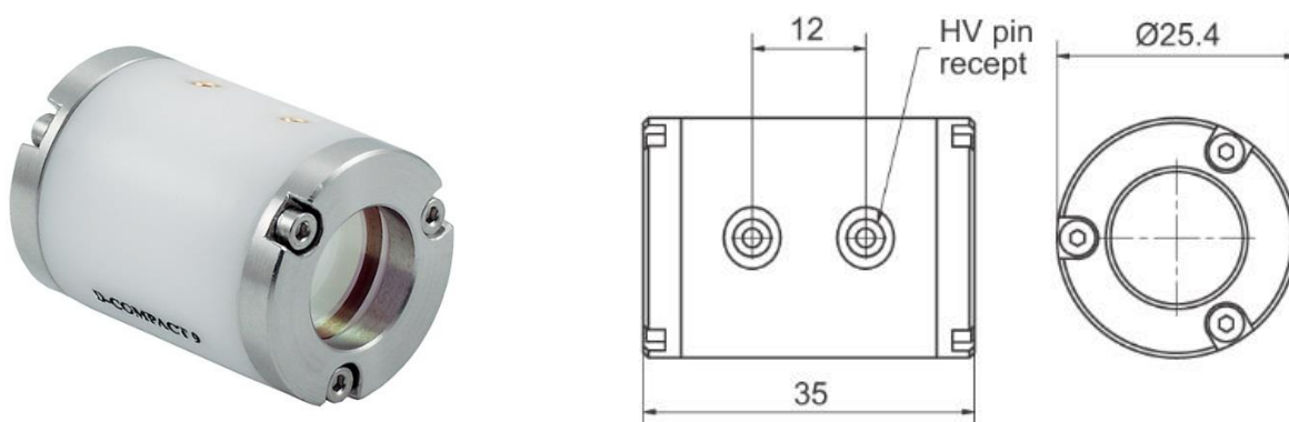
Outline picture and drawing of D-compact/9 DKDP (KD*P) Pockels cell
